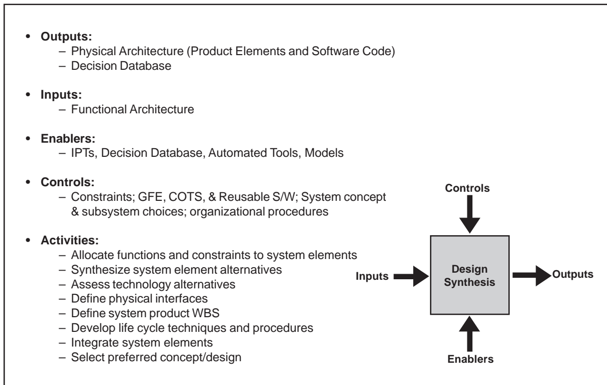
Figure 6-1. Design Synthesis
