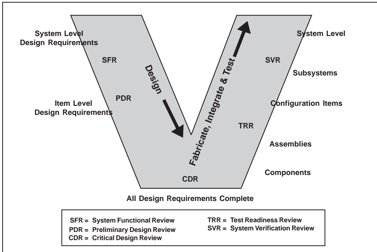
Figure 7-1. Design Synthesis
