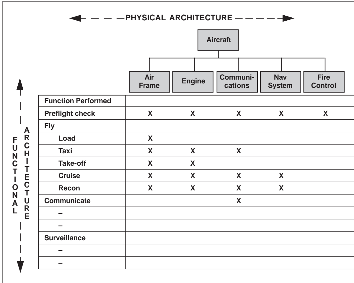
Figure 6–2. Functional/Physical Matrix
