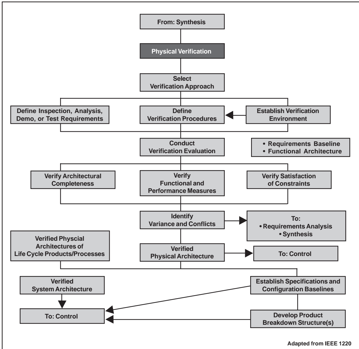
Figure 7-2. Verification Tasks
