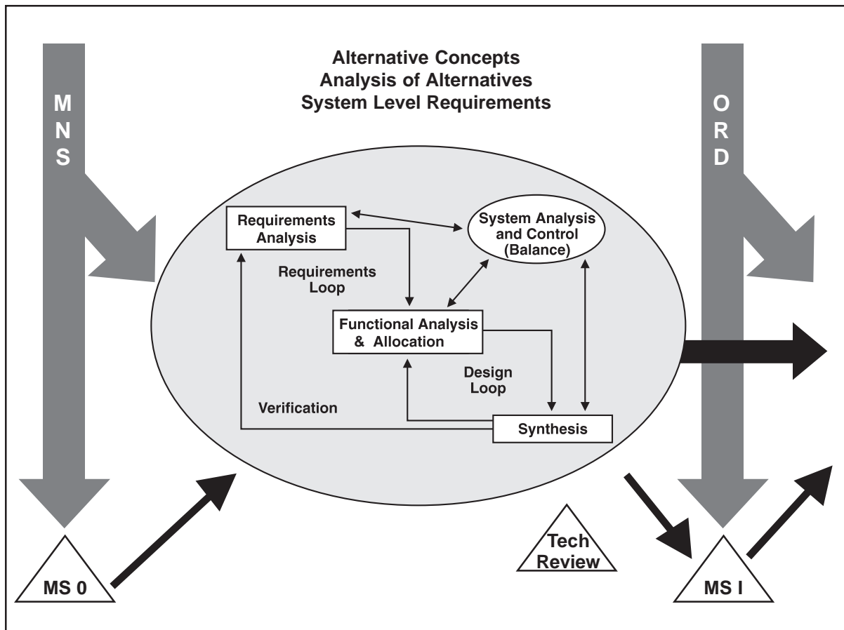
Figure 2-2. Concept Exploration
